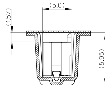
SECT. X-X
