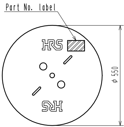
2 Reel style and dimensions
