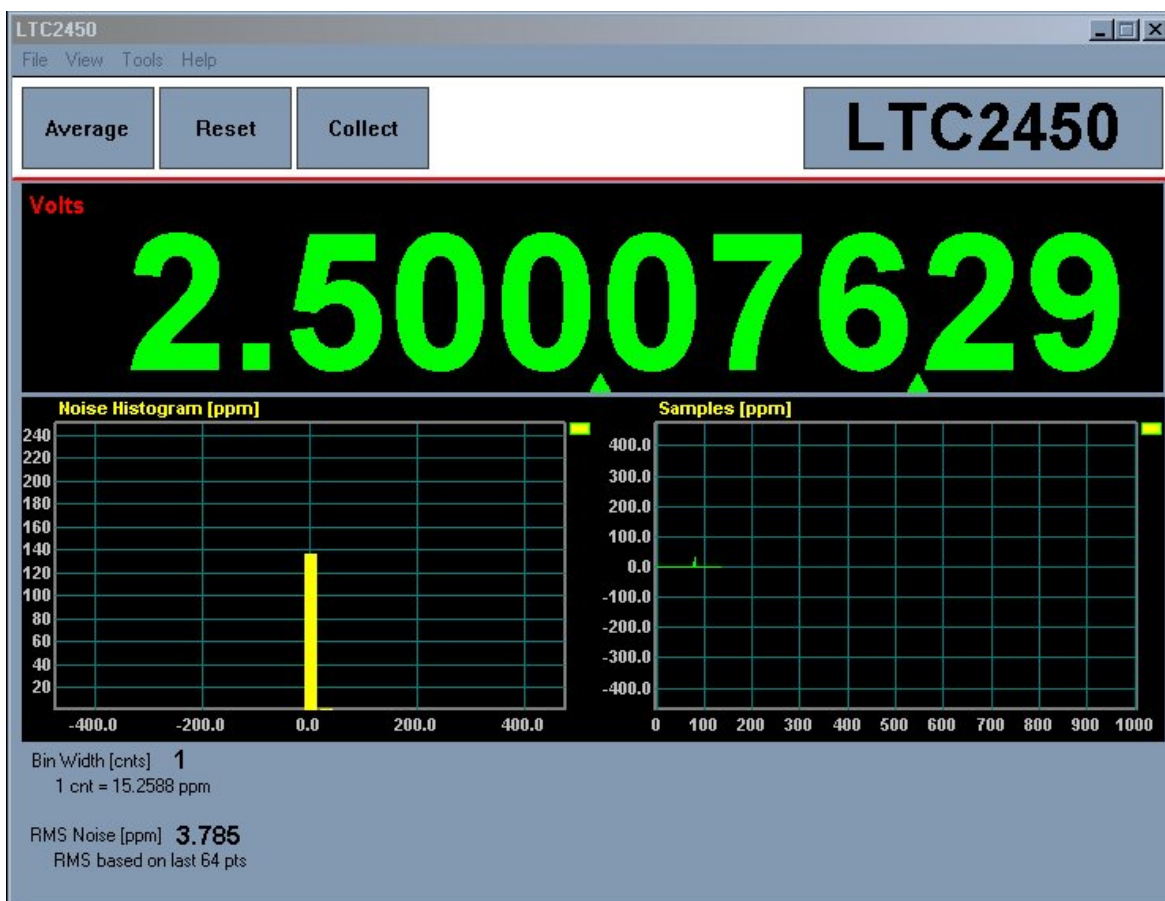
Figure 2. Software Screenshot
