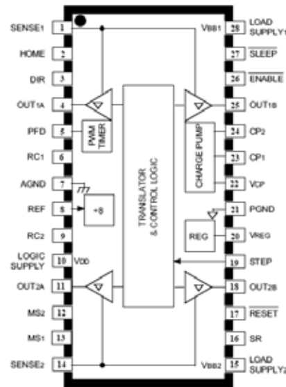
LP Package, 28-Pin TSSOP Pin-out Diagram
