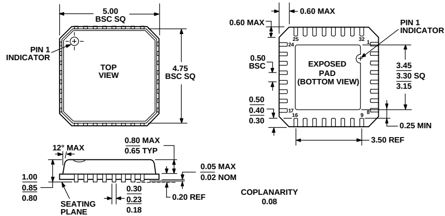
Figure 60. 32-Lead Lead Frame Chip Scale Package [LFCSP] 5 mm x 5 mm Body (CP-32-3) Dimensions shown in millimeters
