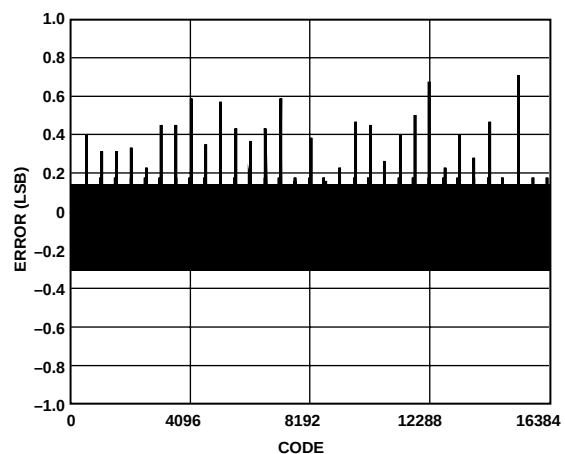
Figure 17. Typical DNL
