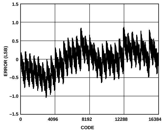
Figure 16. Typical INL
