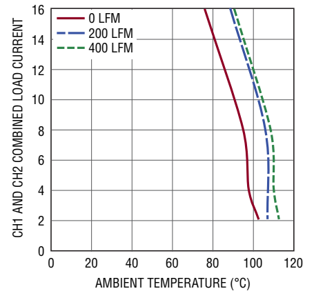
Figure 13. 5V to 1V Derating Curves, No Heat Sink
