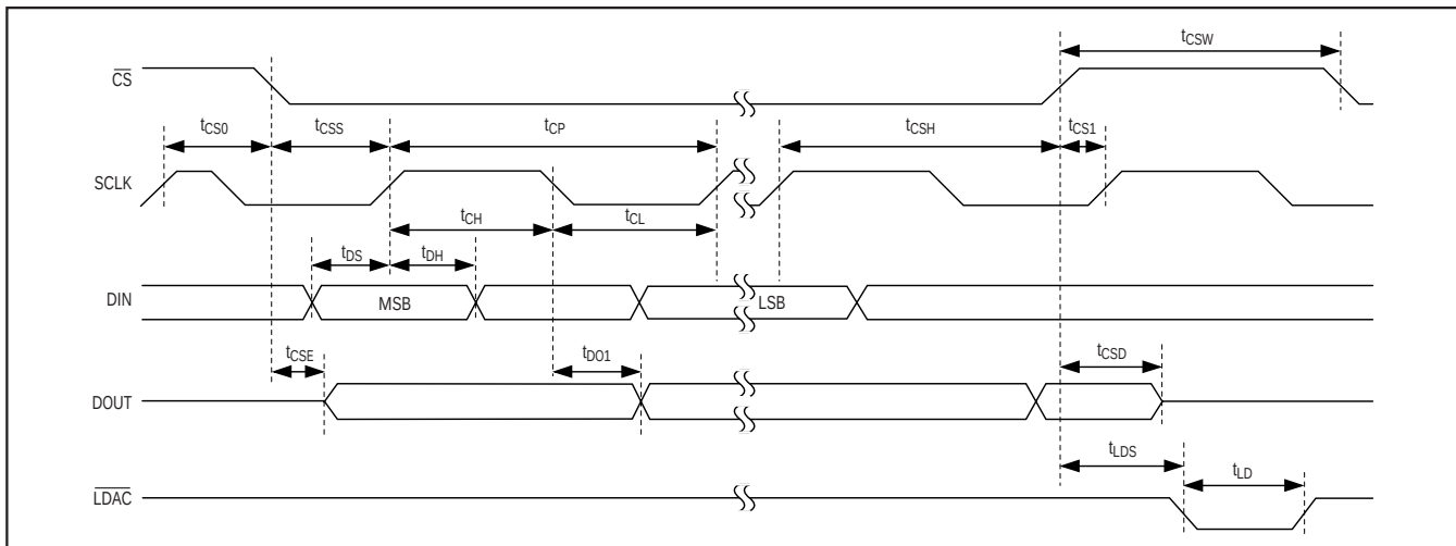
Figure 3. Serial-Interface Timing Diagram
