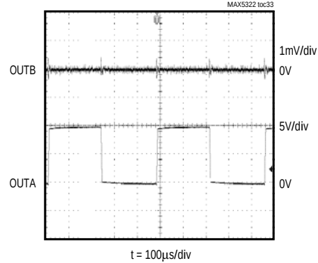
DAC-TO-DAC CROSSTALK
