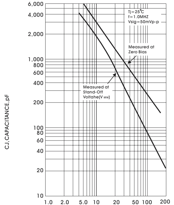
FIGURE 4 TYPICAL CAPACITANCE
