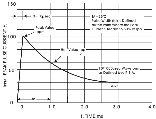
FIGURE 3-PULSE WAVEFORM
