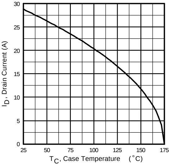
Case Temperature
