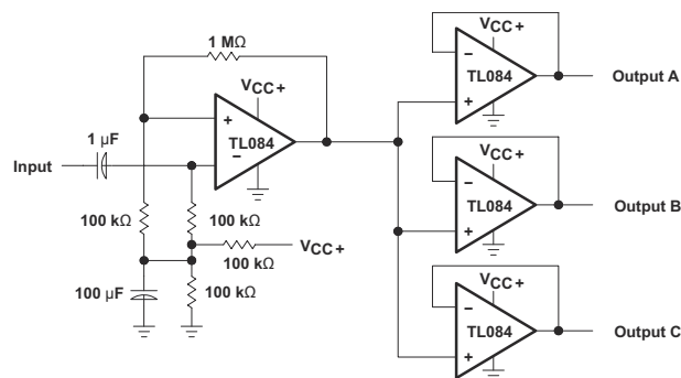
Figure 8-5. Audio-Distribution Amplifier
