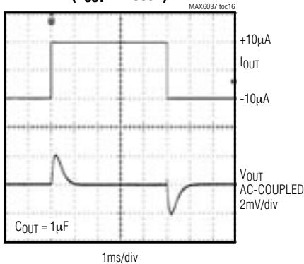
MAX6037_41 LOAD TRANSIENT ( V_{OUT} = 4.096V )
