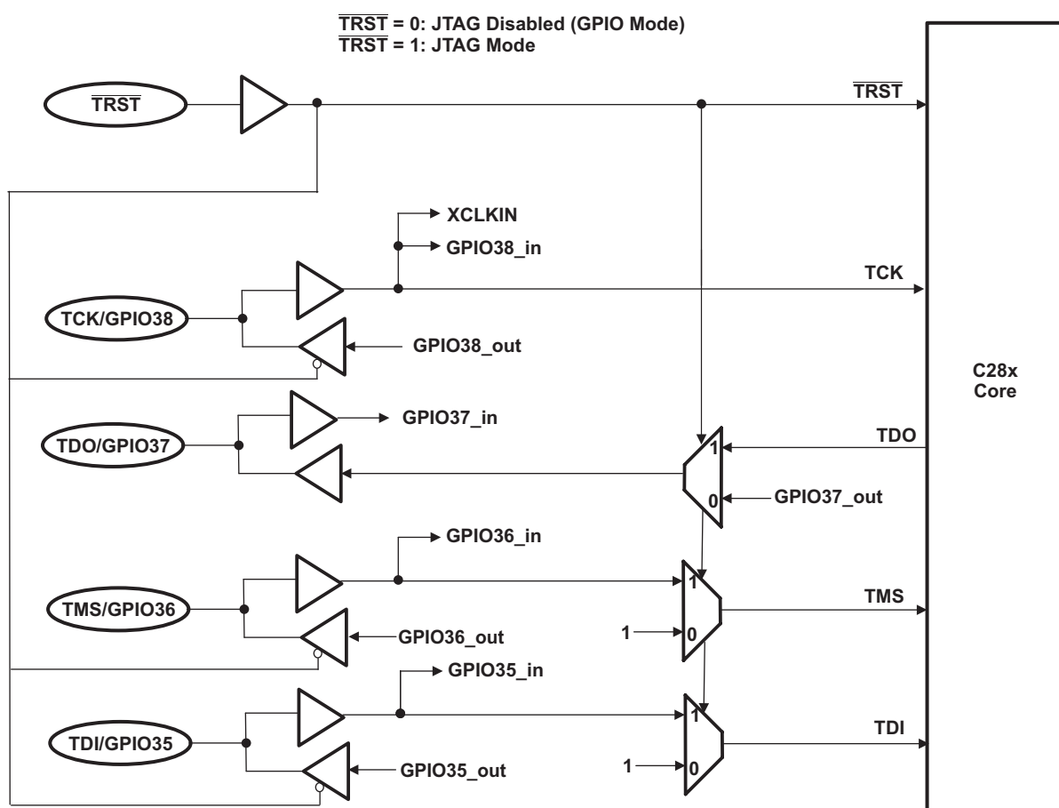
Figure 6-44. JTAG/GPIO Multiplexing
