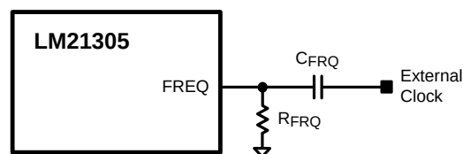
Figure 20. Switching Frequency Synchronized to the External Clock
