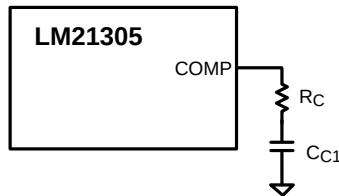
Figure 29. LM21305 Compensation Network
