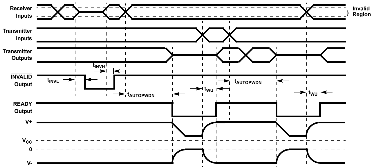
Figure 17. Enhanced Automatic Powerdown, INVALID and READY Timing Diagrams
