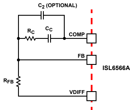
FIGURE 20. COMPENSATION CONFIGURATION FOR LOAD-LINE REGULATED ISL6566A CIRCUIT
