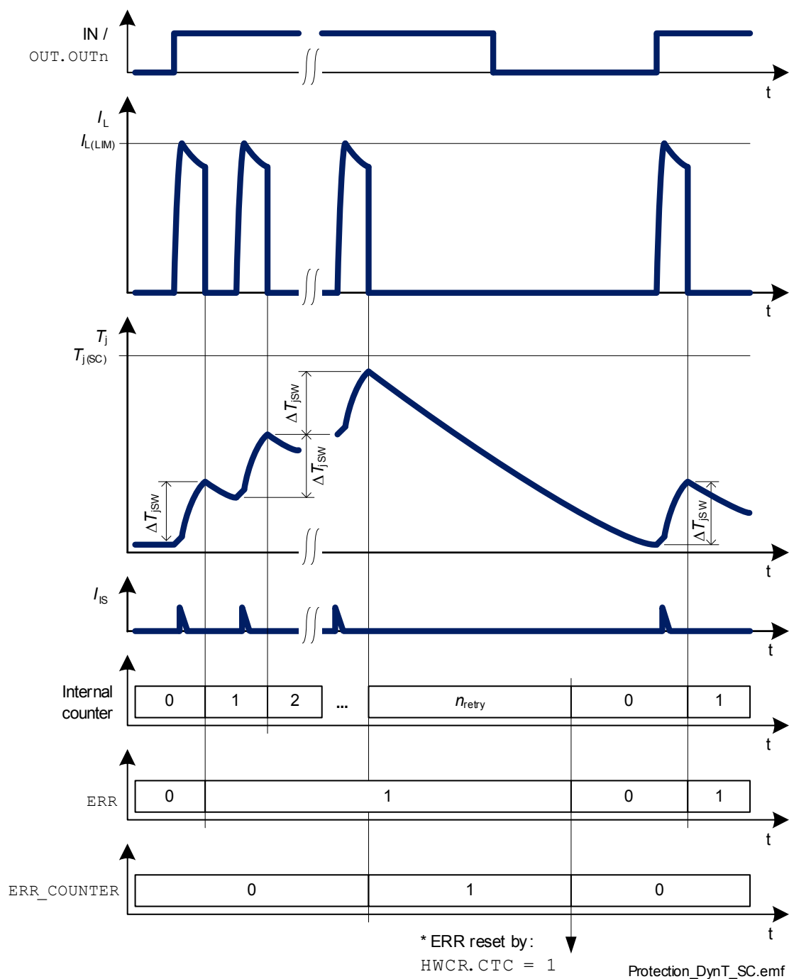
Figure 18 Dynamic Temperature Sensor Operations - Short Circuit
