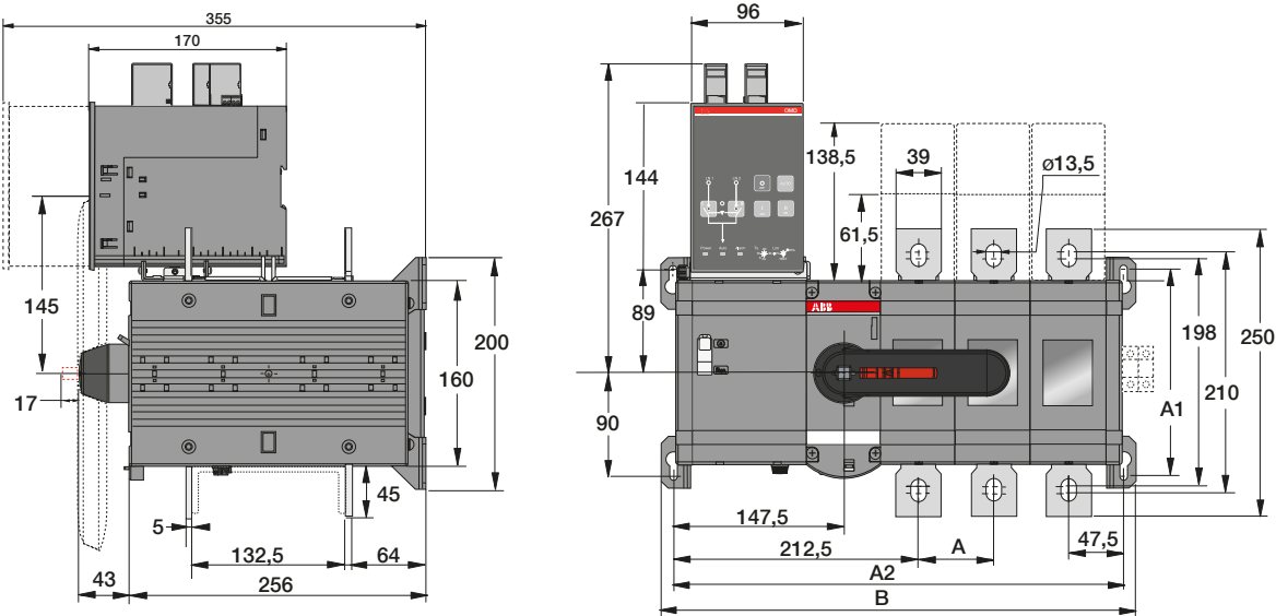
OTM630...800E_C_2D_, OTM630...800E_C_3D_
