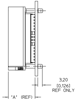
J-LEAD MOUNT
