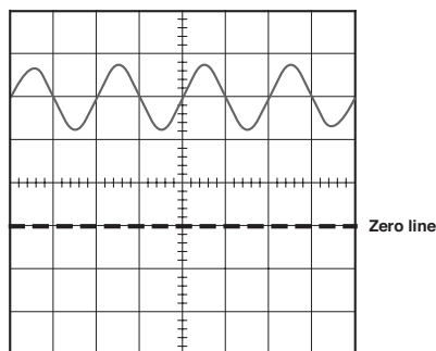
Figure 15. Oscilloscope display showing a typical AC signal superimposed on a DC level from pin 6 of the LM741 in the transmitter circuit.
