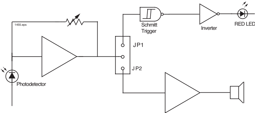
Figure 15. Receiver block diagram.
