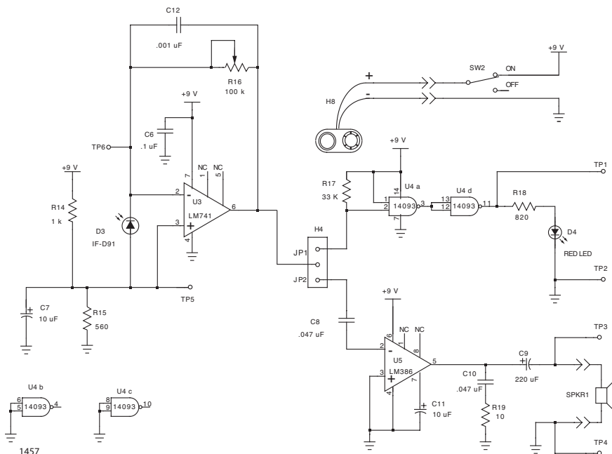
Figure 16. Receiver circuit schematic.
