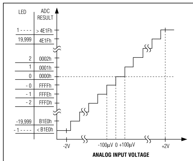
Figure 16. MAX1366 Transfer Function—±2V Range
