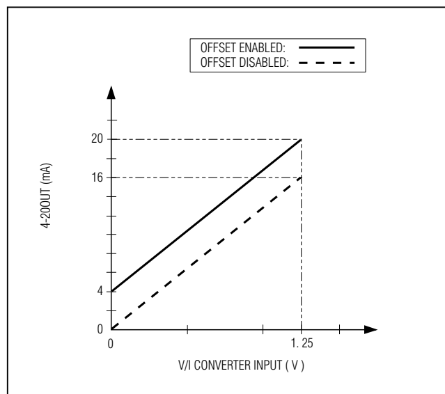
Figure 23. 4-20OUT Output Current vs. V/I Converter Input Voltage
