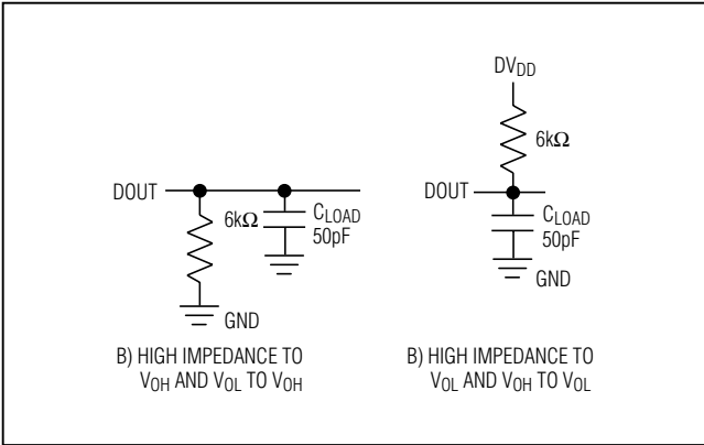
Figure 13. Load Circuits for Enable Time
