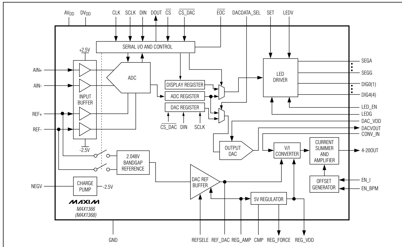
Functional Diagram
