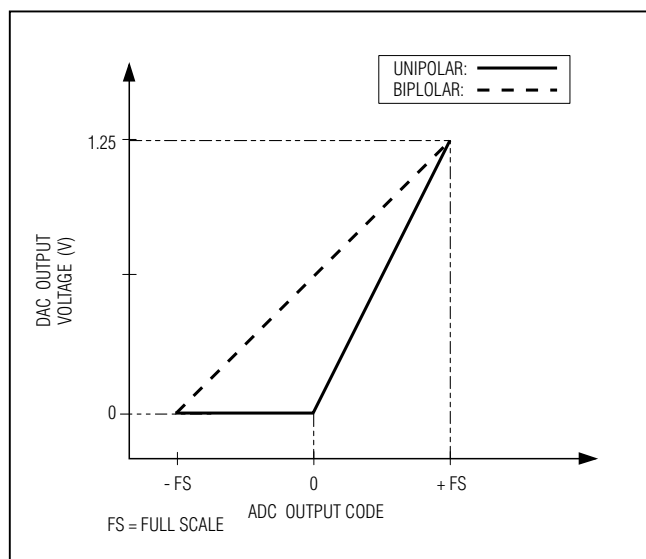
Figure 20. DAC Output Voltage vs. ADC Output Code
