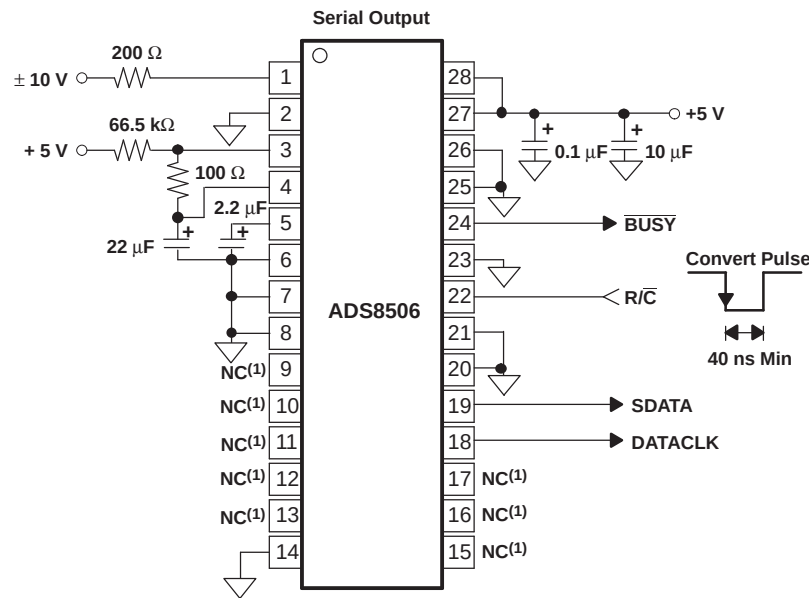
Figure 32. Basic \pm 10 -V Operation With Serial Output
