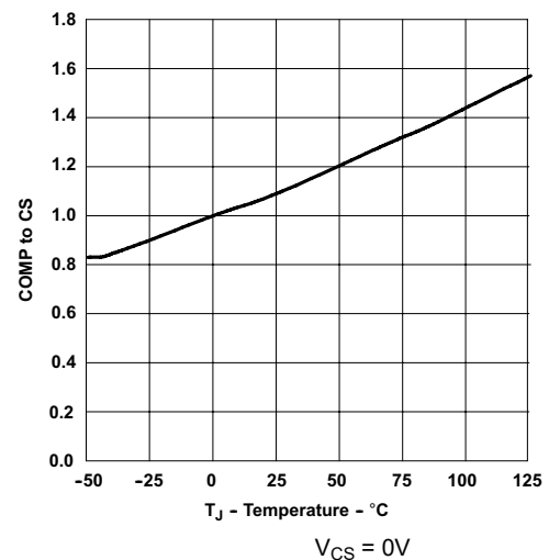
Figure 6-4. COMP to CS Offset Voltage vs Temperature
