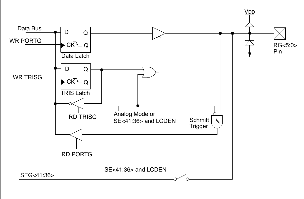
FIGURE 3-29: BLOCK DIAGRAM OF RG<5:0>
