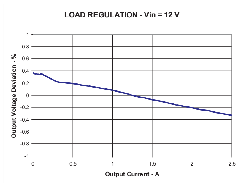
Figure 3. TPS54240EVM-605 Load Regulation
