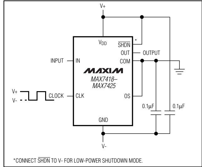
Figure 5. Dual-Supply Operation
