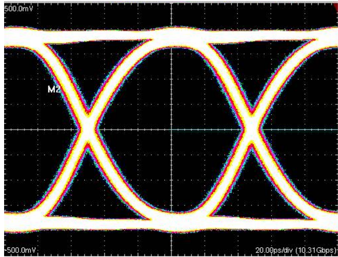
FIGURE 3A. DE-EMPHASIS 0
