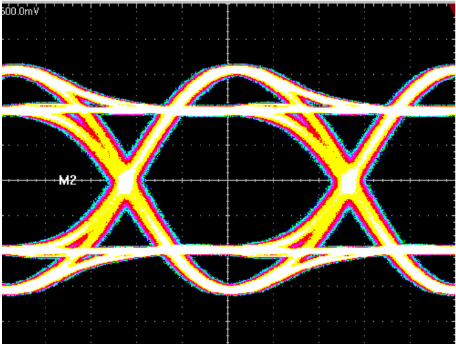
FIGURE 3B. DE-EMPHASIS 6
