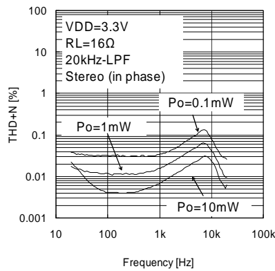
Fig.52 THD+N vs. Frequency (VDD=3.3V, RL=16\Omega )
