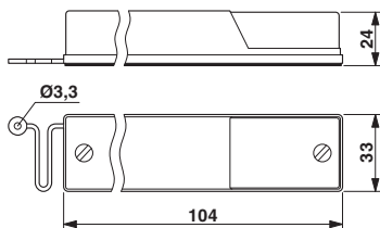
Dimensioned drawing
