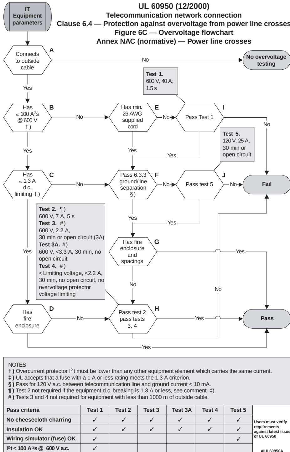
Figure 3. UL 60950 Power Cross Flow Chart
