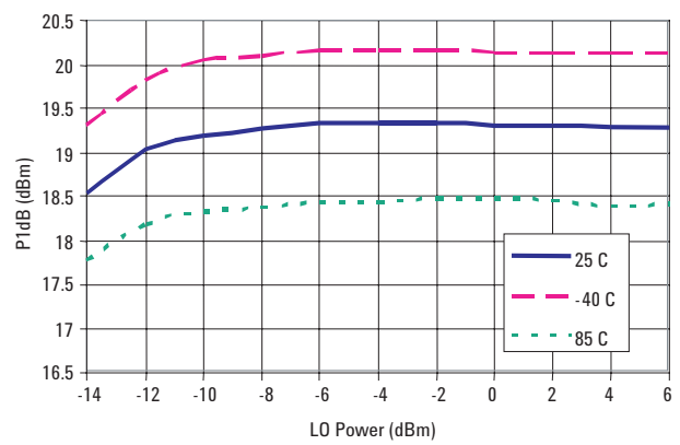
Figure 8. P1dB vs. LO Power and Temperature
