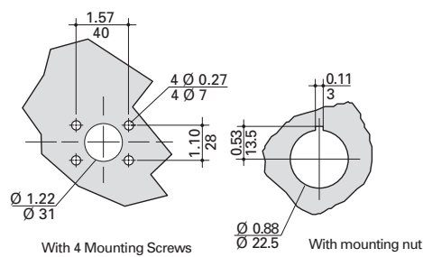
With 4 Mounting Screws With mounting nut
