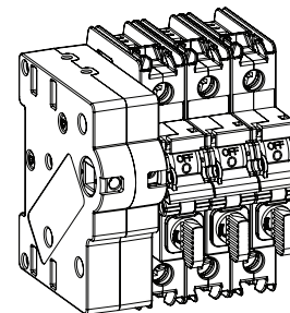
Left side rotary switch
