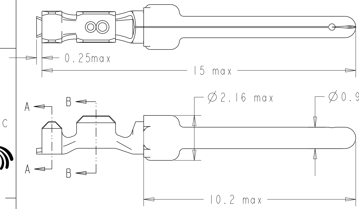
DIMENSIONS FOR MALE & FEMALE
