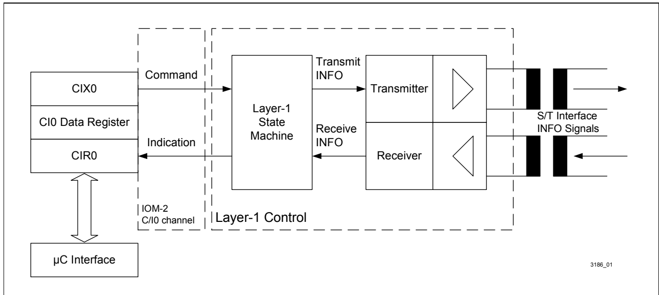
Figure 31 Layer-1 Control
