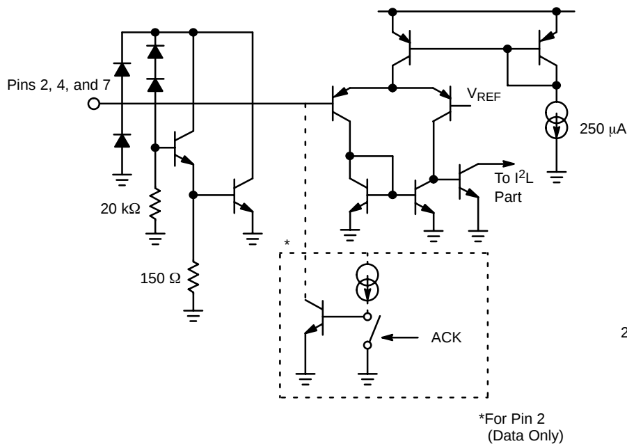
Figure 5. Bus I/O Configuration
