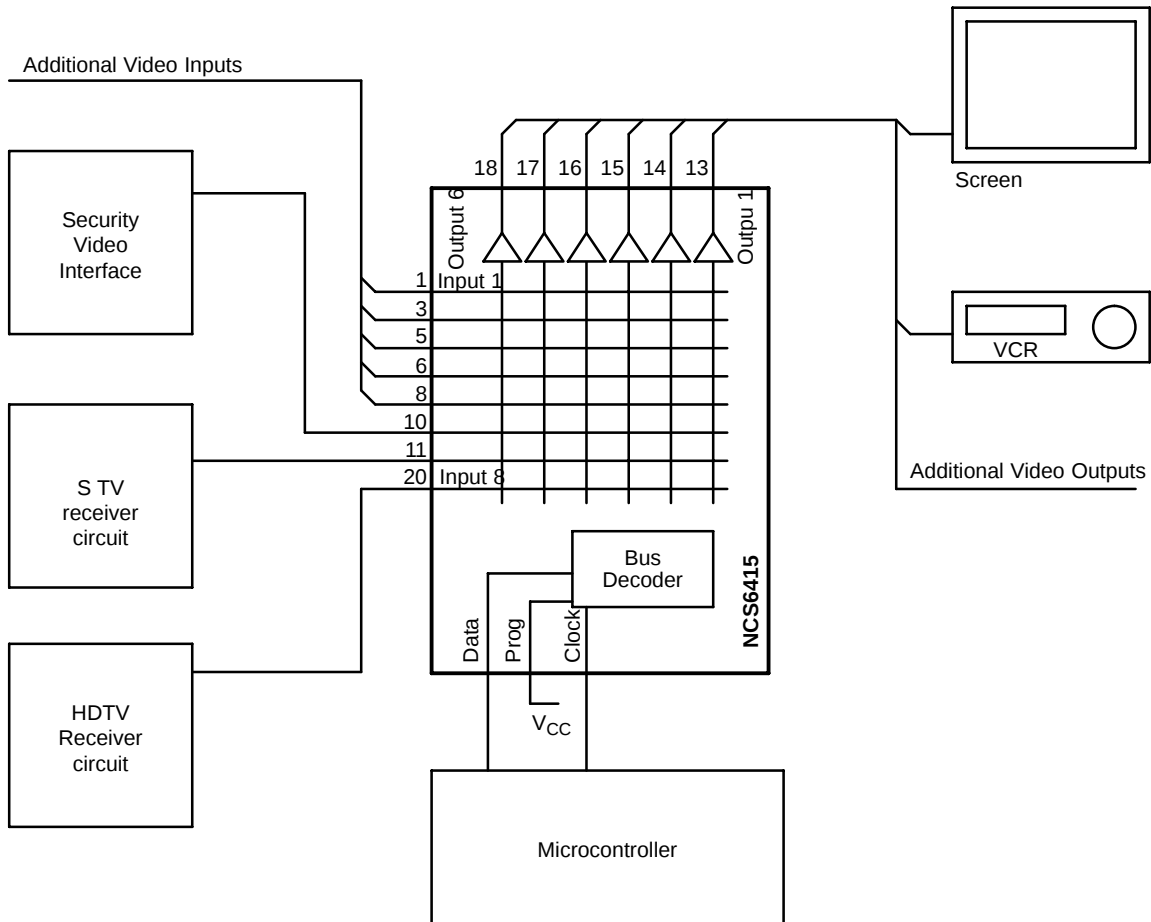
Figure 8. Typical Application Diagram
