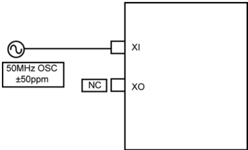
Figure 19. 50MHz Oscillator Reference Clock Connection
