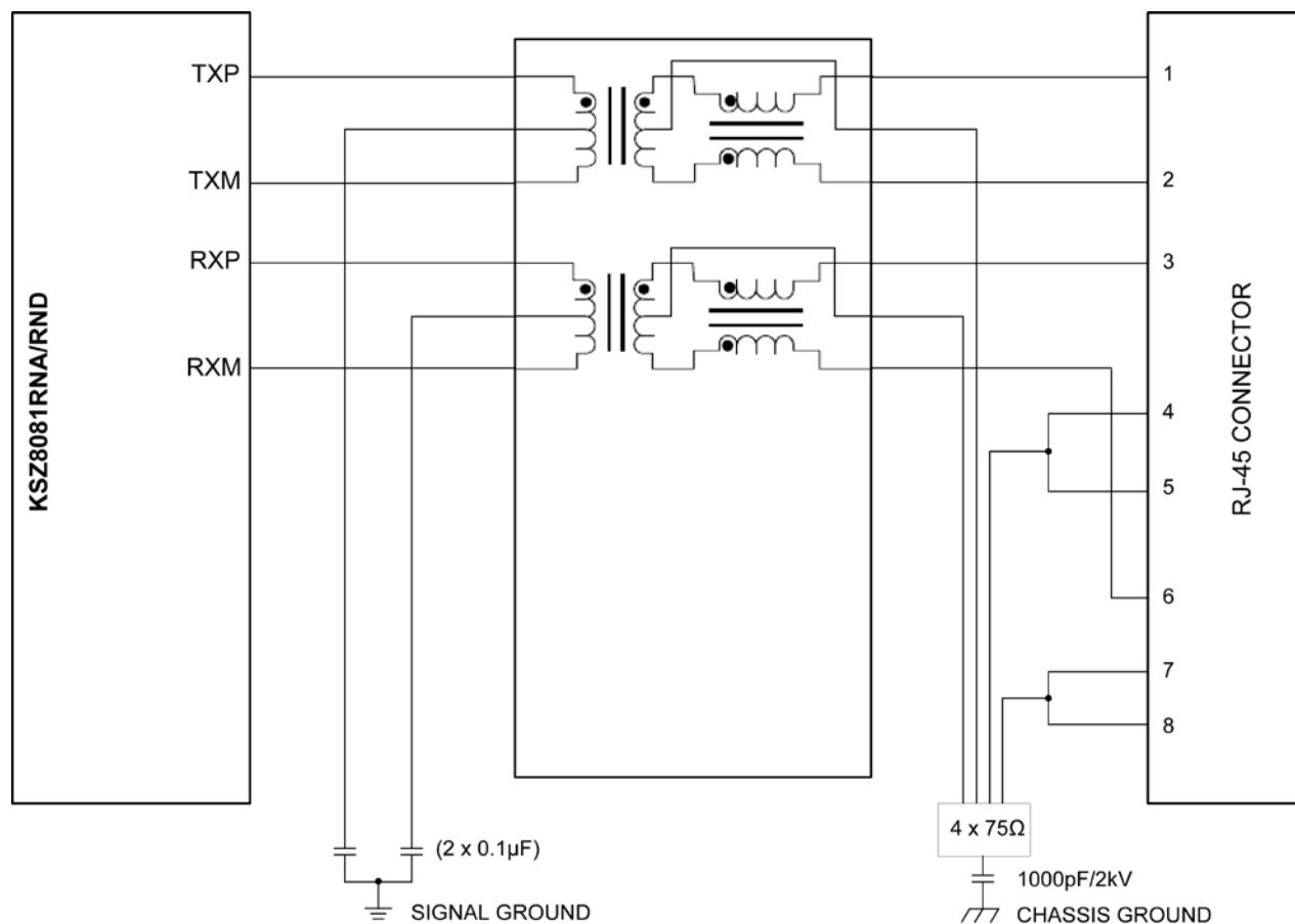
Figure 20. Typical Magnetic Interface Circuit
