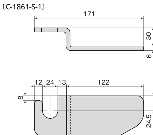
掛け金(左用) Hook (For the left-hand use)
