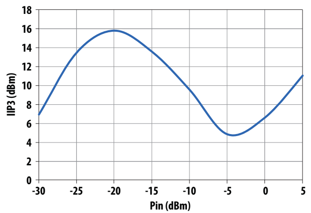
Figure 35. Bypass Mode IIP3 vs Input Power
