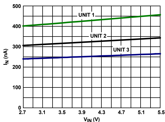
FIGURE 14. I_{IN} vs V_{IN} , THREE UNITS
