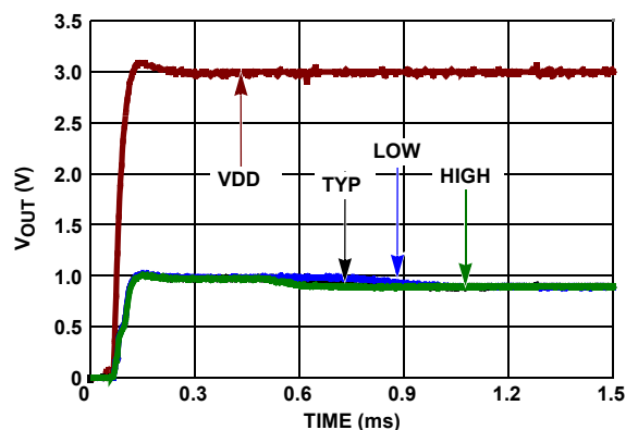
FIGURE 13. TURN-ON TIME
