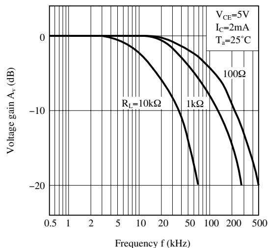
Fig.15 Frequency Response
