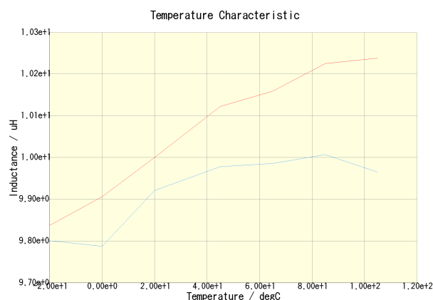
VLF403215MT-100M-CA(DC = 0A)
