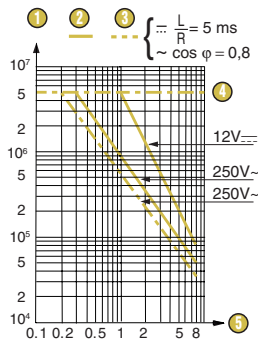
Operating curve for type 831690
