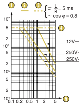
Operating curve for type 831694
