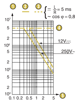
Operating curve for types 831698/831699
