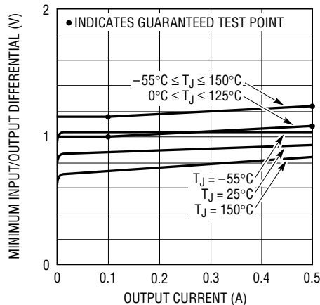
LT1086H Dropout Voltage
