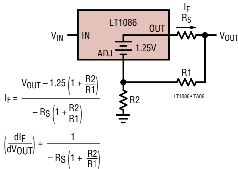
Battery Charger
