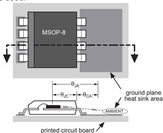
Figure 1. Thermal Resistance
