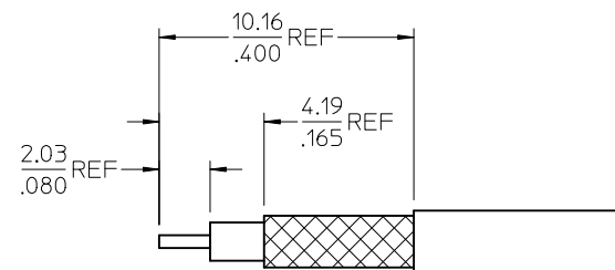
RECOMMENDED STRIP DIMENSION CRIMP SIZE: .128 HEX
