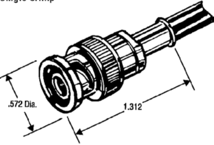
Single Crimp
