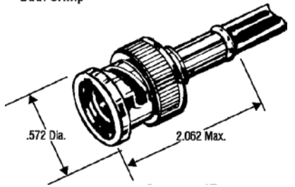
Dual Crimp
