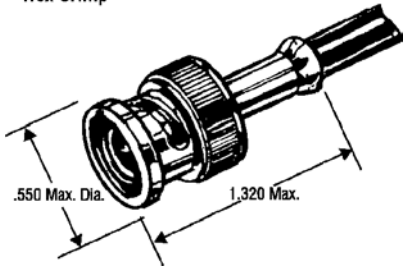
Hex Crimp
