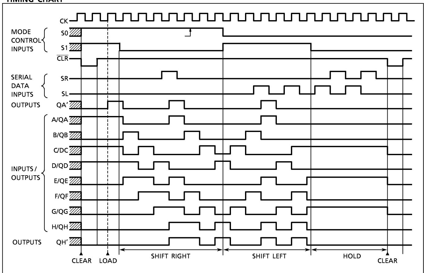
TIMING CHART
