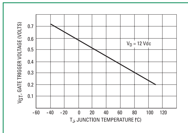
Figure 4. Gate Voltage
