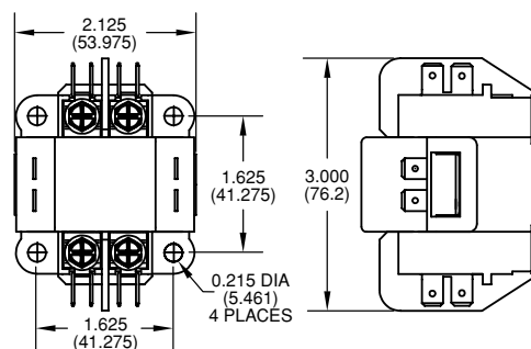
Model 2000-20 (two pole)
