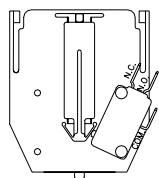
ONE SPDT SWITCH PER SIDE
