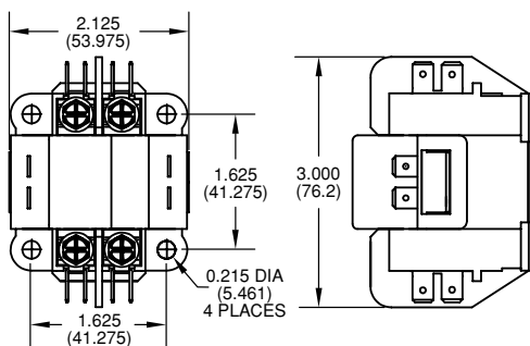
Model 2000-10 (one pole) Model 2000-15 (one pole with shunt)
