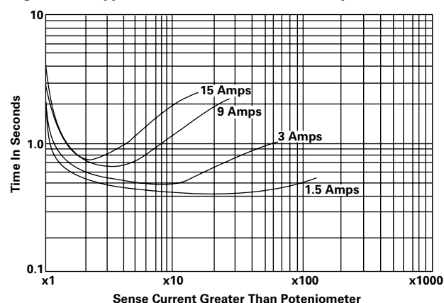
Figure 1 – Typical Overcurrent Time Delay Curves
