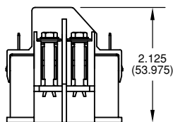
Model 2000-10 (one pole) Model 2000-15 (one pole with shunt)
