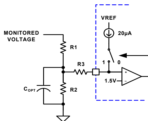
FIGURE 13. OV HYSTERESIS
