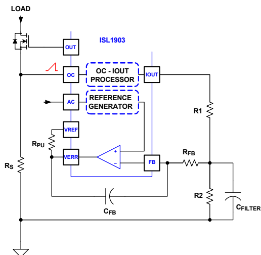
FIGURE 11. CONTROL LOOP CONFIGURATION
