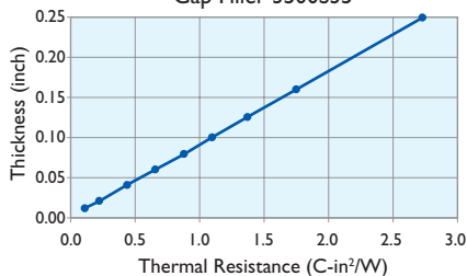
Thickness vs. Thermal Resistance Gap Filler 3500S35
